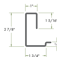
Gable Clip 18 Ga. Galv. Steel 18 Ga. Stainless Steel
